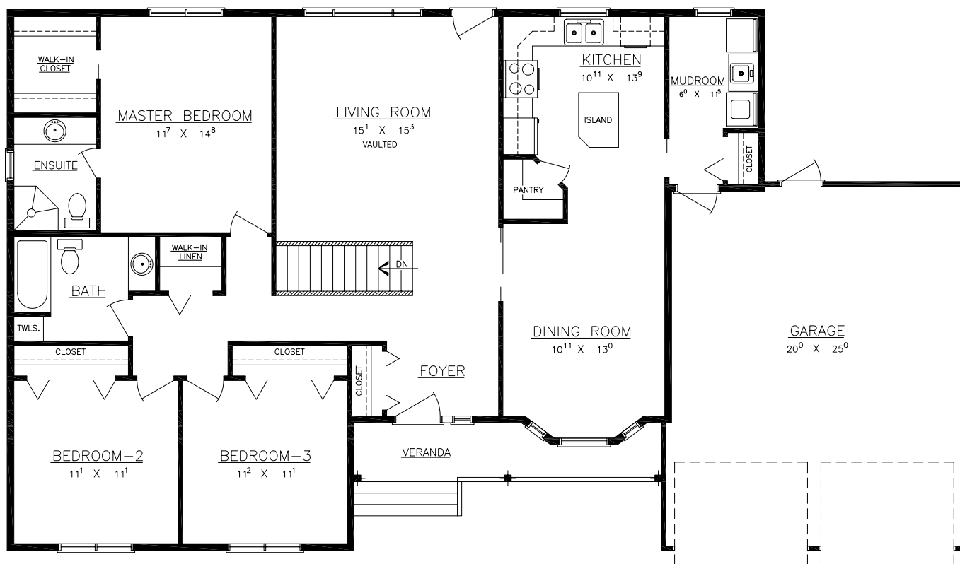
FLOOR PLAN
